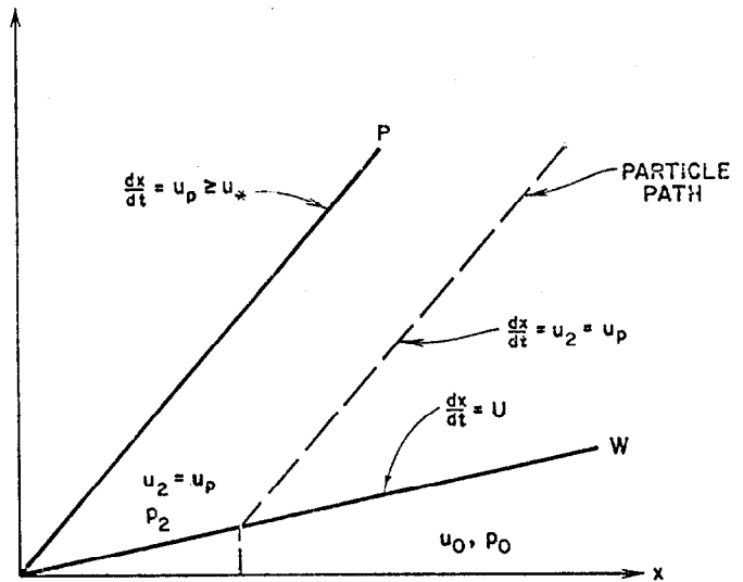
FIG 1 Flow in a strong detonation. Piston path (P), detonation front (W), and particle path (dashed) are shown
